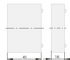
Contenitori da parete Surface-mounted housing
