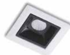
PROJECTOR LED SINKRO-2M BR/PR 2W 45° 160Lm 4000K 4,5x4,5x4,9cms
