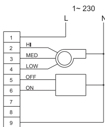
Fans with heating and cooling three-way SPDT valve system
