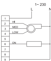
Ventilation with heating and cooling two-way SPST valve system
