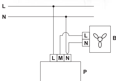
Controller wiring diagram
