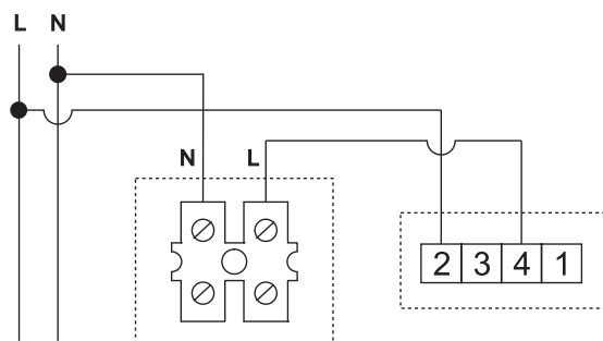
Fan starts operation as the temperature reaches the threshold value set by the thermostat.
