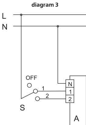
Fan is manually switched to one of two speeds by speed switch S (f.e. P2-1-300) or switched off.
