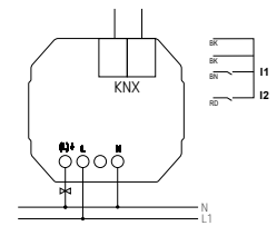
LUXORliving H1
