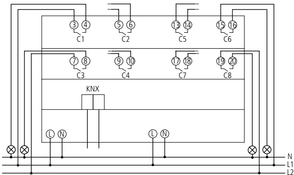
RM 8 | KNX
