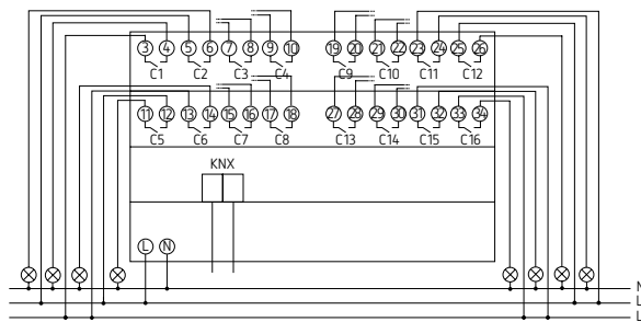
LUXORliving S16
