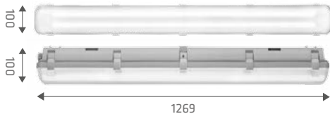
CODAR RS LED EVO ENDURA MINUS 60W
