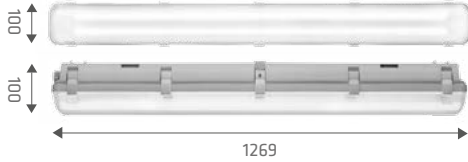
CODAR RS LED EVO ENDURA PLUS 28W
