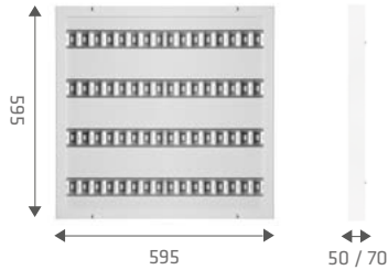
595x595x50 - dimension variant I 595x595x70 - dimension variant II
