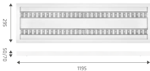
295x1195x50 - dimension variant I 295x1195x70 - dimension variant II
