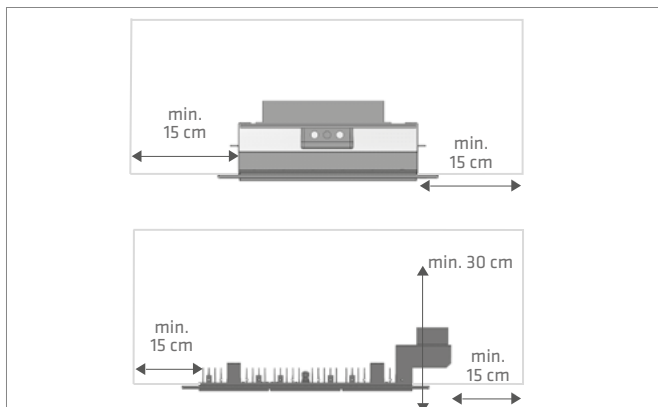
Mounting dimensions
