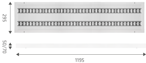
295x1195x50 - dimension variant I 295x1195x70 - dimension variant II
